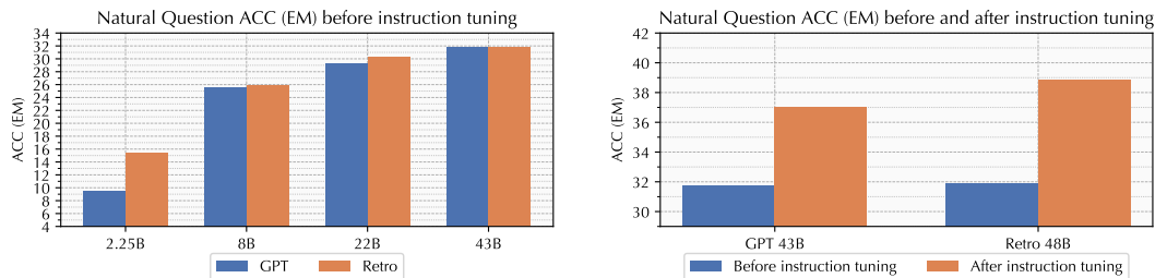
(a) Before instruction tuning, the improvement of retrieval augmentation saturates when the size scales up.
