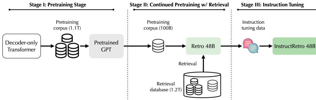
Figure 1: Training pipeline for InstructRetro 48B.
