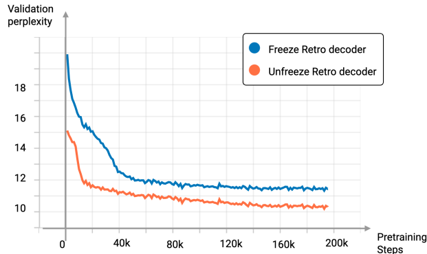
Figure 3: Validation perplexity of Retro-fitting when we freeze or unfreeze Retro decoder during continued pretraining on 100B tokens.
