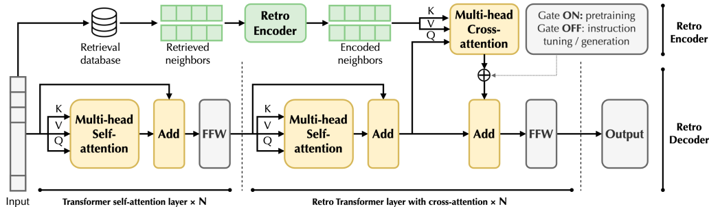
Figure 4: Retro simplified architecture diagram. We omit the layer norm, softmax, and embedding layers for simplicity. We add additional 0/1 gates between cross-attention output and the residual connection from self-attention output. During pretraining, we keep the Retro encoder gate ON (one). During instruction tuning and inference, we turn the Retro encoder gate OFF (zero) when there is no retrieved neighbors.
